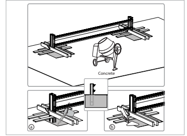
Concrete footing installation
